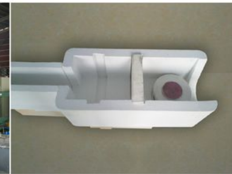
透气砖除气流槽 Porous brick launder degassing equipment
